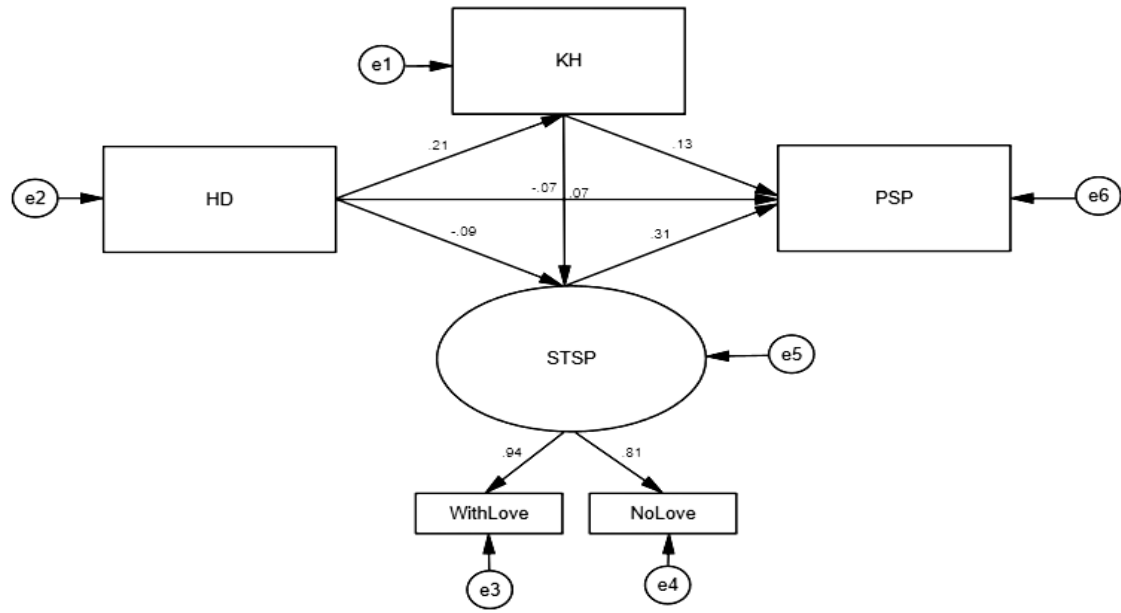
Gambar 1. Model Empiris
